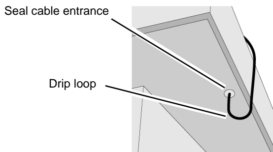
FIG-7: Outside Antenna Cable Installation
